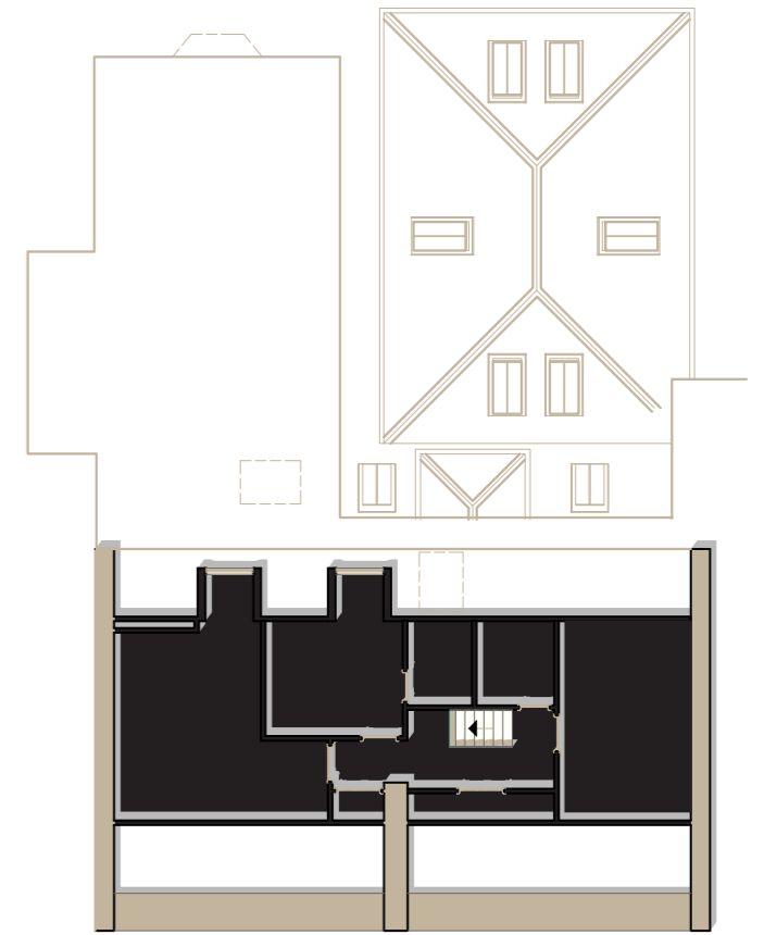
ATTIC
